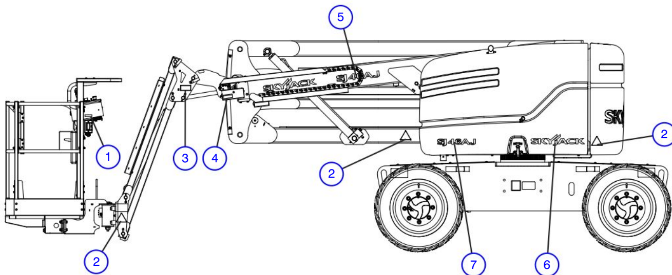
Engine Side
